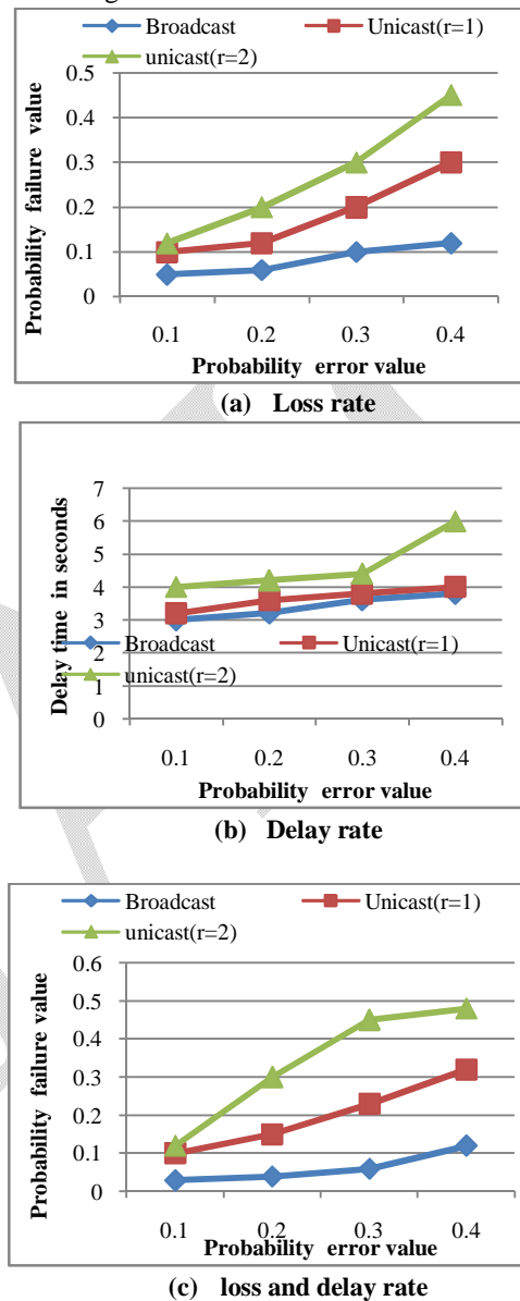
Fig.1. Loss rate and delay information rate
